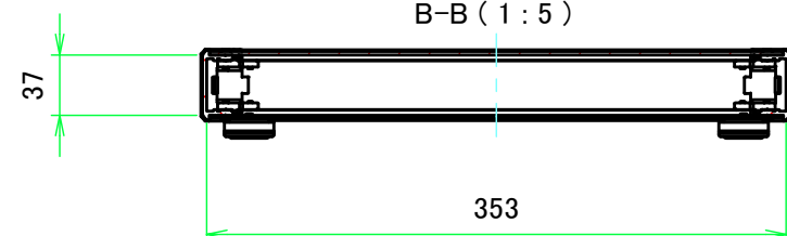
B-B (1:5)
