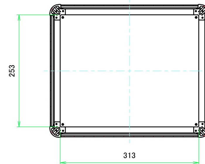
C-C (1:5)
